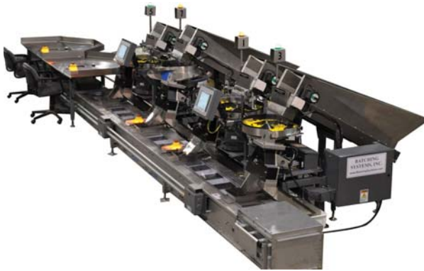
Kit Line with Counters, Bagger, and Conveyor
