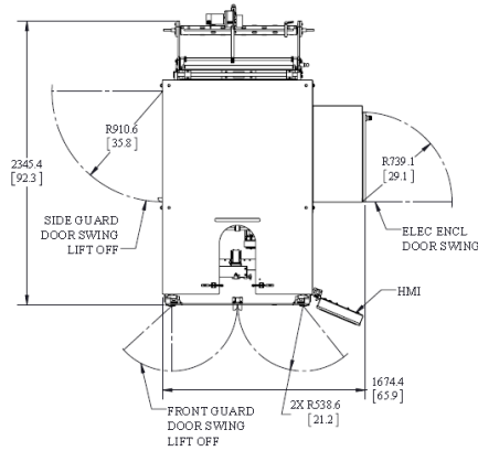
Machine Footprint—Top View
